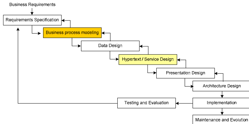
Fig. 1. Development process extensions for SOA
