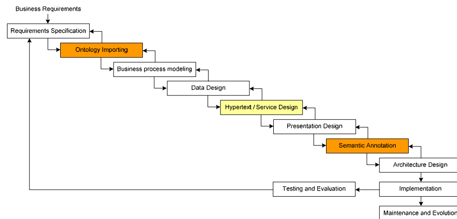
Fig. 5. Development process extensions for SWS
